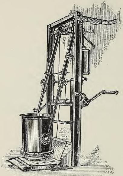
FIG. 21.—Weber's Elevator, First Position.
